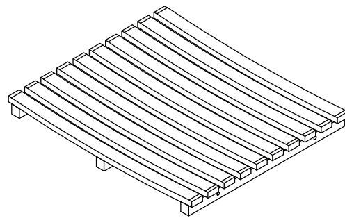
4 SEAT PANEL X 1PC
