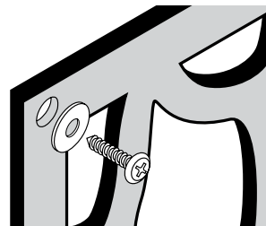
OVERSIZED HOLE WITH PAN HEAD SCREWS
