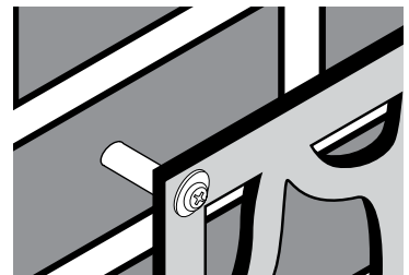
OVERSIZED HOLE WITH SPACER AND PAN HEAD SCREWS
