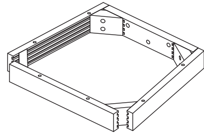
(B) Seat Frame (1PC)
