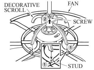
4. Install the scroll assembly to the fan.
