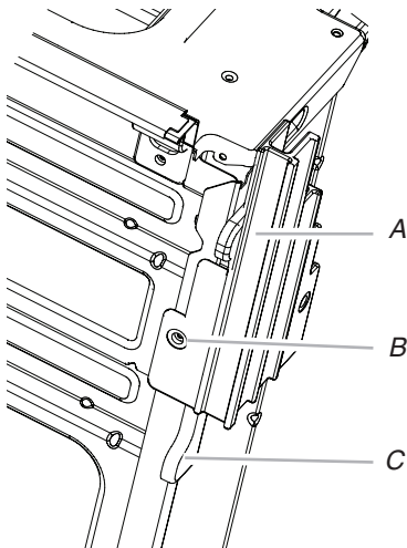
A. Front foot B. #8-18 x \frac{3}{8} " (9.5 mm) screw C. Spacer
