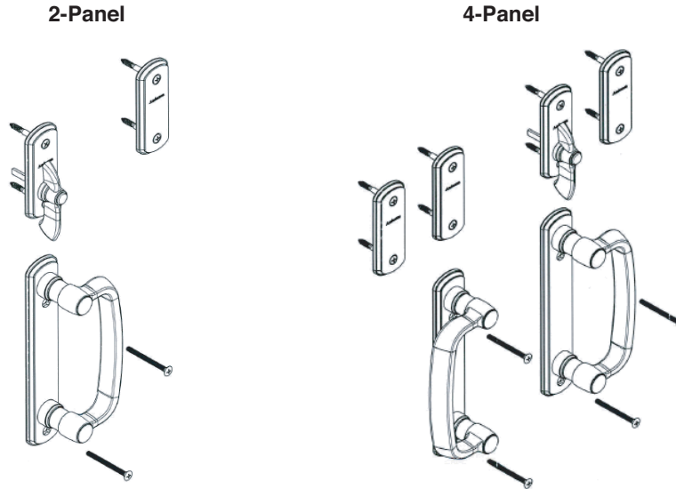
RH Handle, Albany Style Shown
