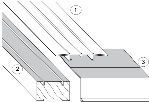
Frenchwood® Gliding Support Mullion
