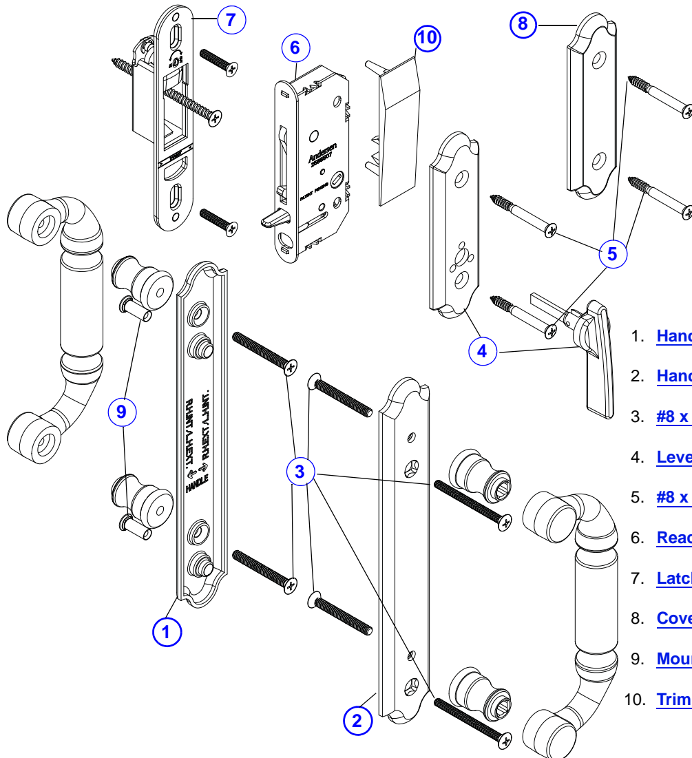
Covington™ Gliding Patio Door Hardware - 2-Panel Trim Set
