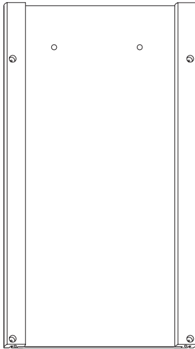
Side Panel (2) P/N SP/HDL-51538
