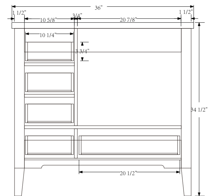
BACK VIEW
