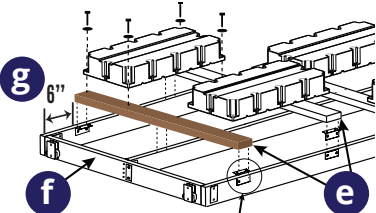
OPTIONAL CORNERS TO STRENGTHEN SQUARENESS
