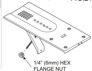
Platform Assembly FIG.21
