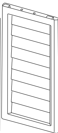
2-05-811
