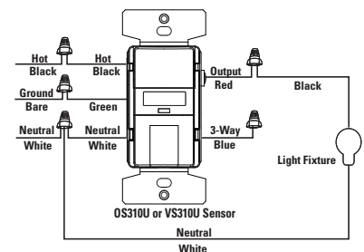
DIAGRAM 1: SENSOR IN ONE LOCATION
