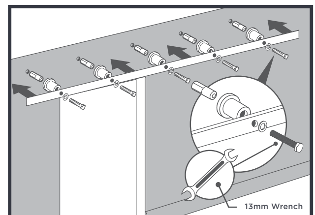
FIGURE 5. Track mount
