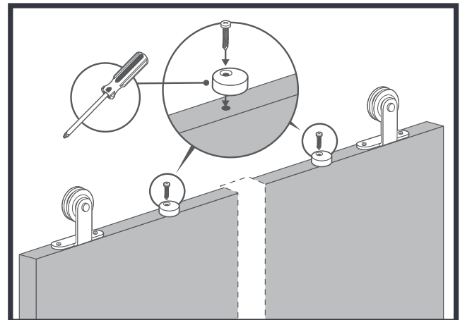
FIGURE 2. Anti-jump blocks installation
