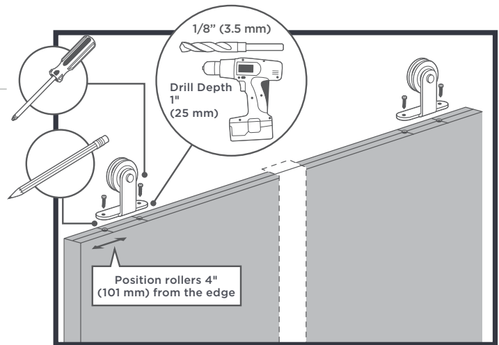
FIGURE 1. Roller Installation
