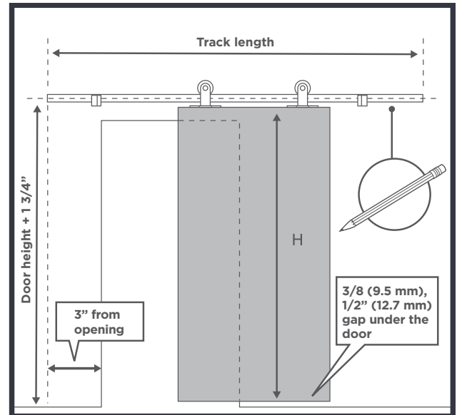
FIGURE 3. Locate the position of the track
