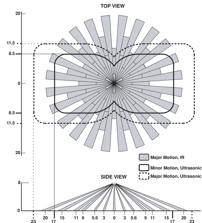
Figure 3 (Cat. No. OSC10) Field-of-View Ranges
