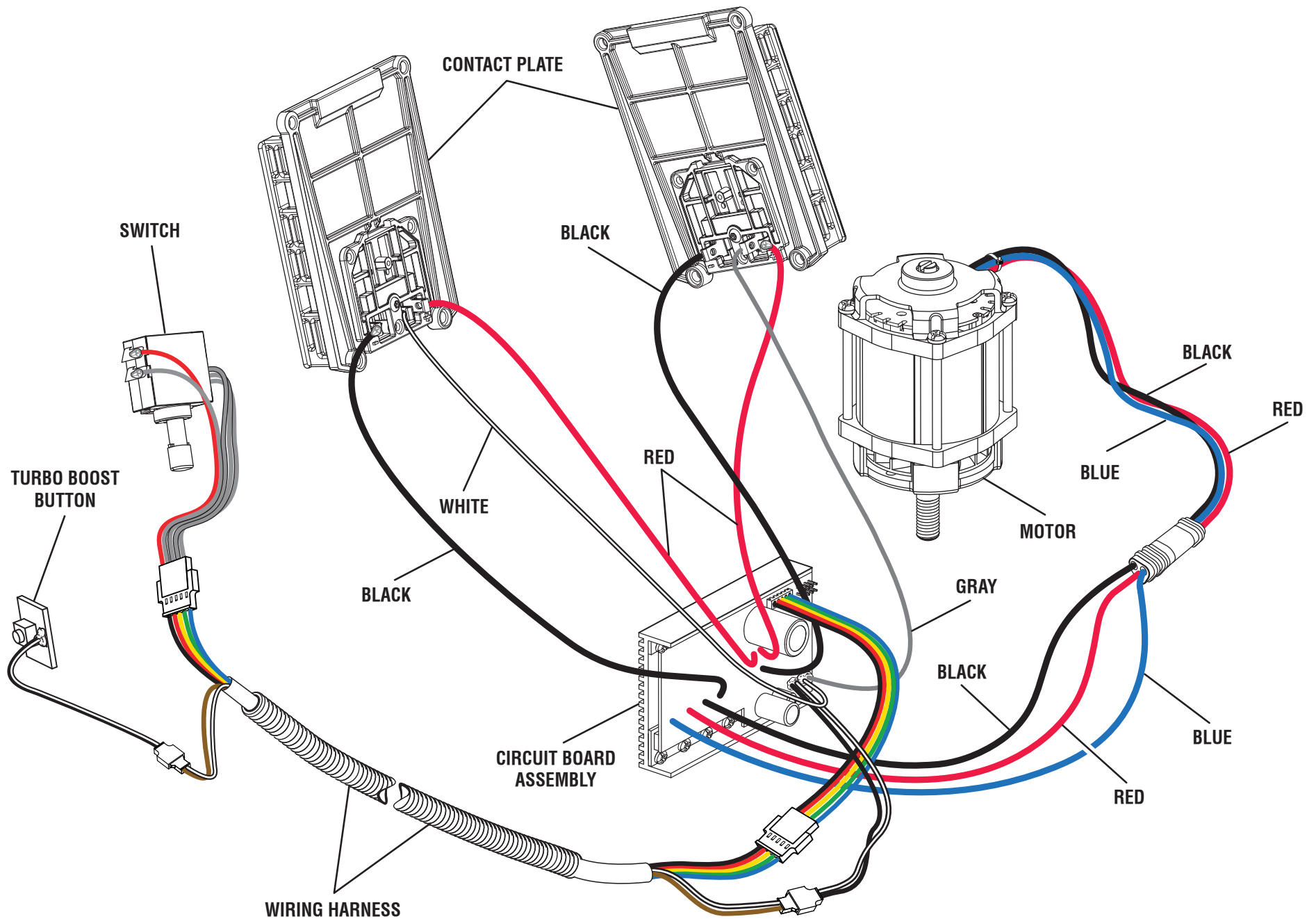
WIRING DIAGRAM
