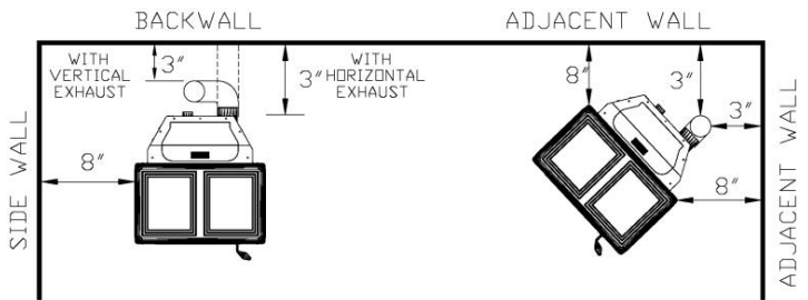
MINIMUM SIDEWALL CLEARANCES
