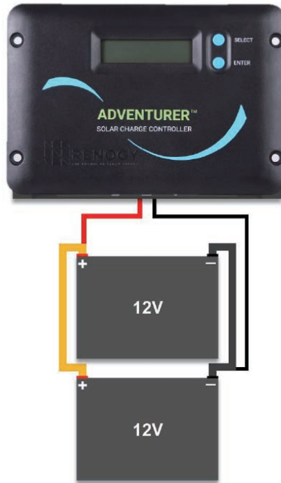
Figure 9.2 Two 12V batteries connected in parallel
