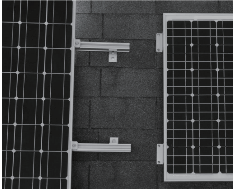
Rail mount vs. Z-Bracket
