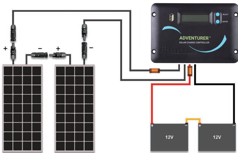
Figure 7.1 Completed 24V off-grid system
