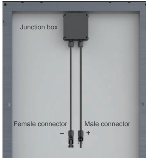
Figure 5.2 Back view of RNG-100D
