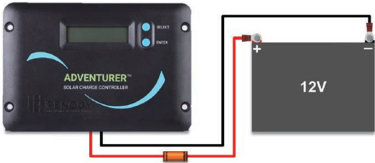
Figure 6.1 Charge controller connected to a 12V battery
