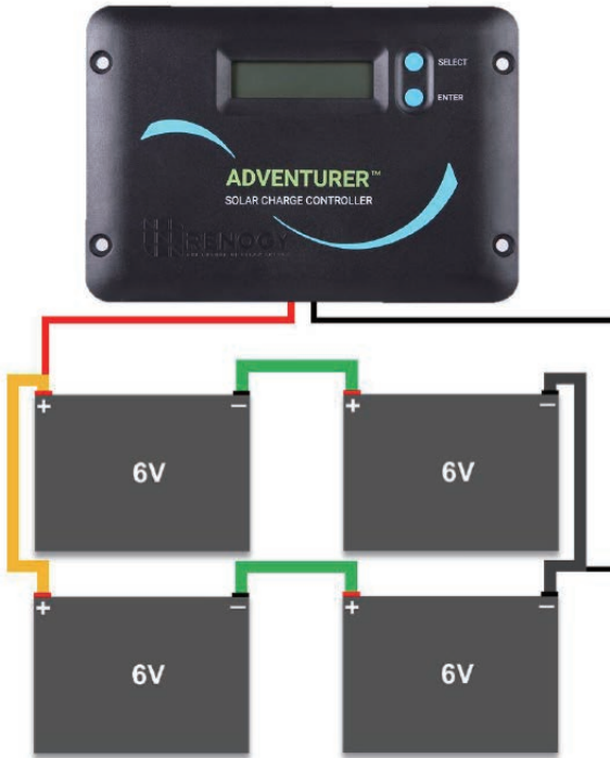
Figure 9.3 Four 6V batteries connected in series – parallel
