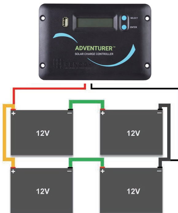
Figure 9.6 Four 12V batteries connected in series – parallel
