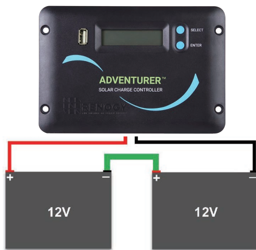
Figure 9.4 Two 12V batteries connected in series
