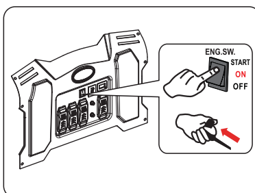
Fig 13 Recoil Start
