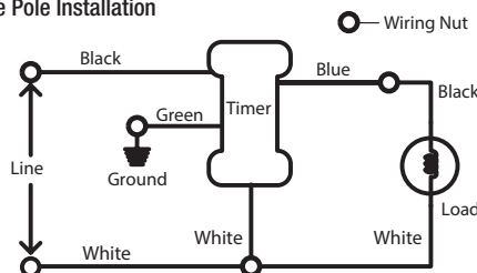
Figure 1 - Typical Wiring Schematic for Single Pole Installation
