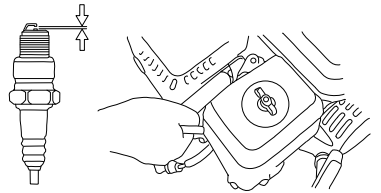
Figure 4-8. Spark Plug
