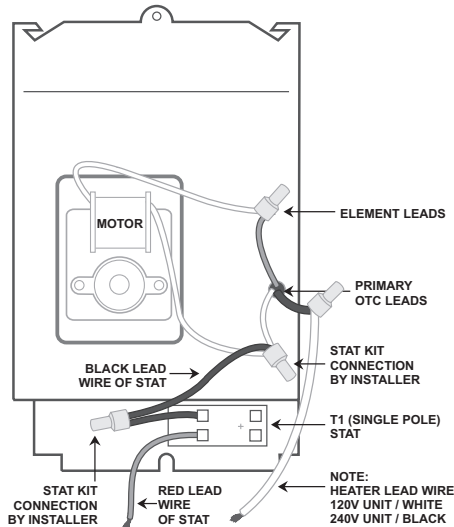
CS Model Single Pole Thermostat (T1)
