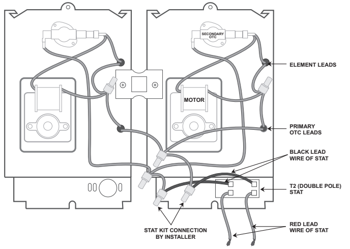
CT Model Double Pole Thermostat (T2)
