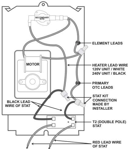
C Model Double Pole Thermostat (T2)
