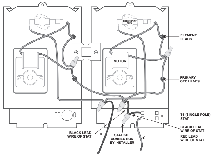
CT Model Single Pole Thermostat (T1)
