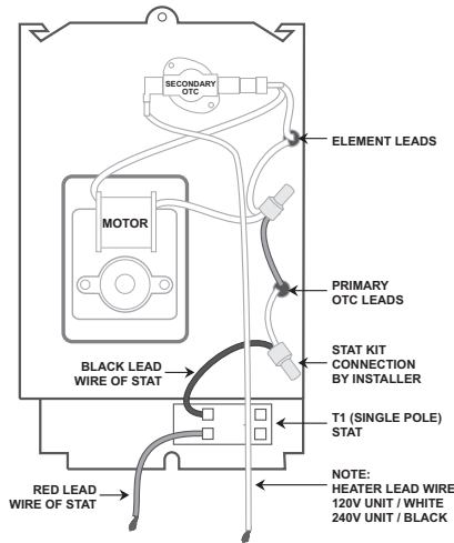
C Model Single Pole Thermostat (T1)
