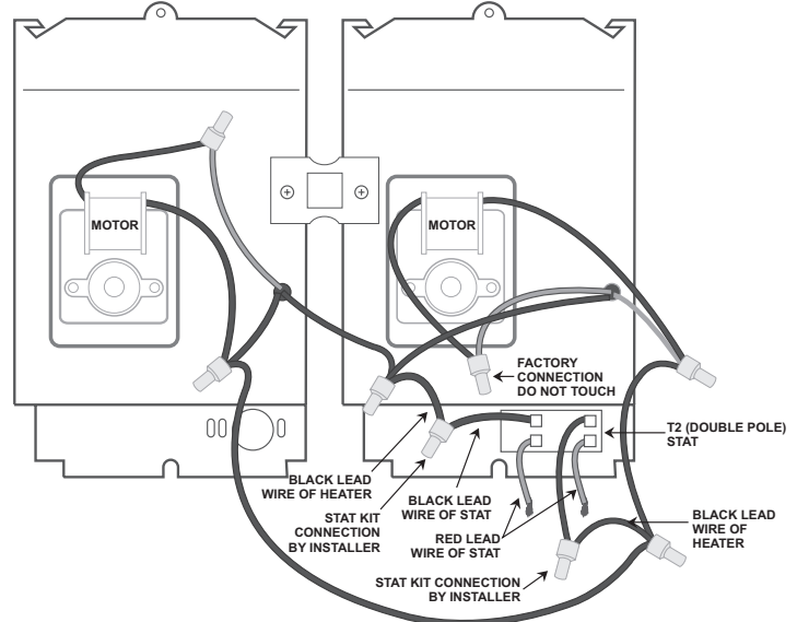
CST Model Double Pole Thermostat (T2)
