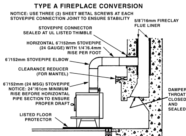
Figure 14 - Fireplace Conversion
