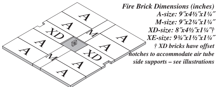
Figure 7a – Step 1, Bottom Firebrick Arrangement Eight (8) A-size, Two (2) M-size, Two (2) XD-size
