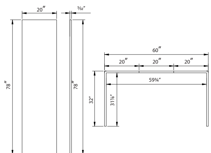
Back Panel Dimensions
