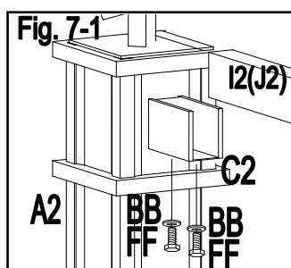
Fig.7-1: Fix Short beam I2, Long beam J2 and Beam connector C2 by using FF, BB.
