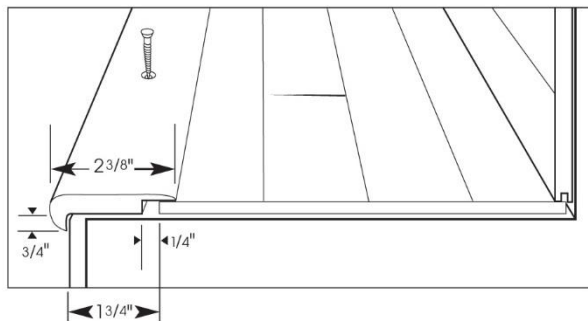
STAIR NOSING
