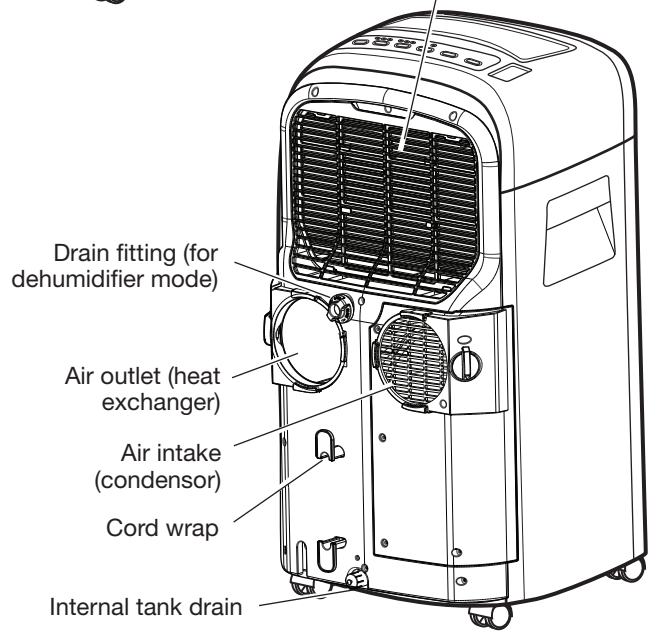
Back View (dual vent models)
