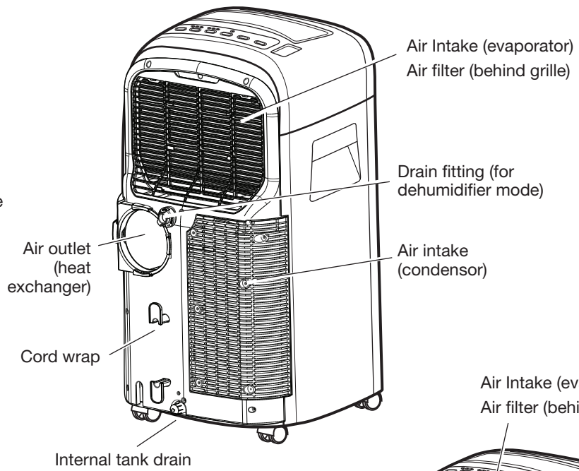
Back View (single vent models)
