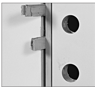
Figure 14: Shims are placed above and below the dead bolt hole (points G in figure 12).
