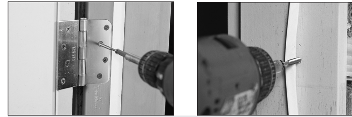
Figures 22 and 23: The second set of supplied screws should be installed under the weather-stripping as shown in Figure 23. It is strongly recommended that you remove the weather-stripping to ensure that you do not pierce or puncture it.
