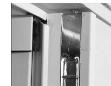
Figure 17: Correct sagging until the flush bolt slides freely into the pre-drilled hole (not typical of most units) in the head/threshold.
