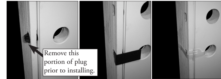
Figure 5: Some door units may be supplied with a clip or plug holding the panel aligned and closed during the initial installation steps. Do not remove at this time. Some door units may be supplied with a double headed nail or screw holding panel closed - this needs to be removed at this time.
