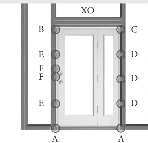
Figure 21: Install shims in the correct location and in the correct sequence.
