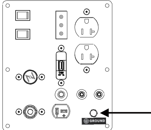
Figure 3 - Attaching the Grounding Wire to this Generator
