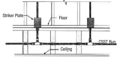
Figure 4.7 Multiple Outlets Along Main CSST Run
