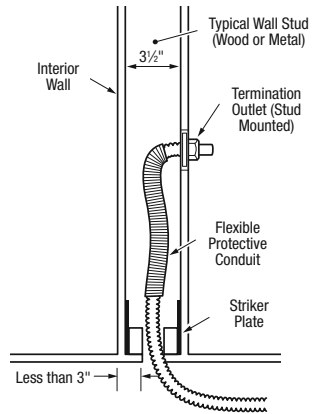
Figure 4.11 Use of Flexible Protective Conduit
