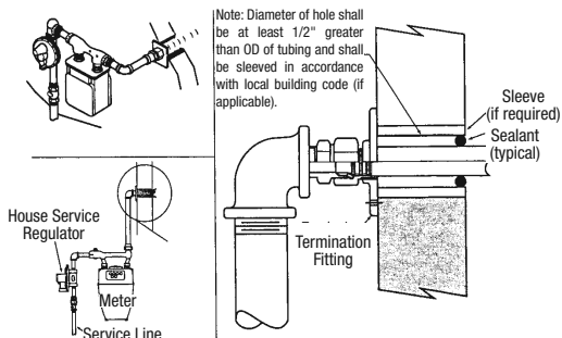
Figure 4.13 Connection to Building supported Meter
