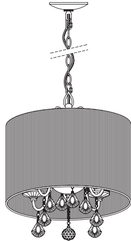
Assembled Fixture
