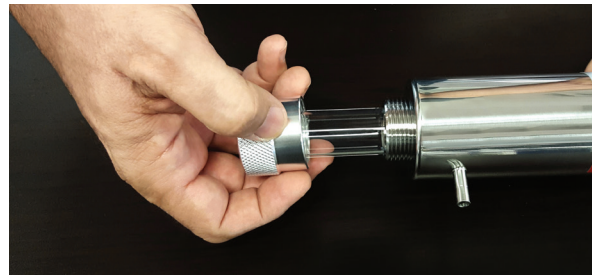
4. Carefully insert the closed end of the Quartz Tube into the open end of the UV Housing with the Metal Cap over the end.
