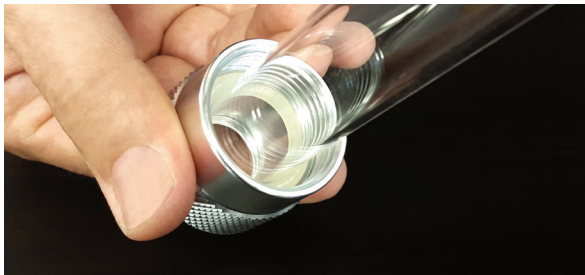
3. Insert the open end of the Quartz Tube into the Metal Cap. The O-Ring will rest against the cap.
