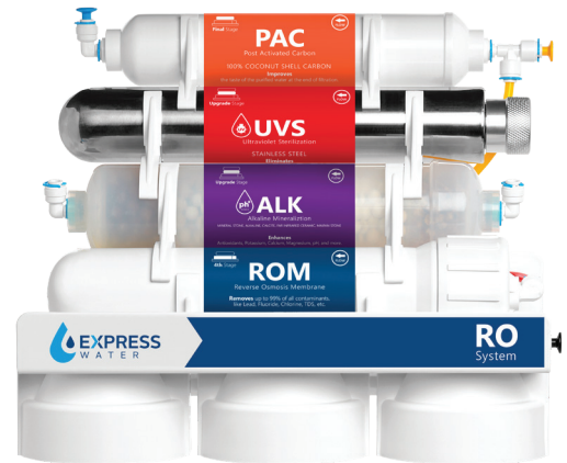
Top Part of the Unit
