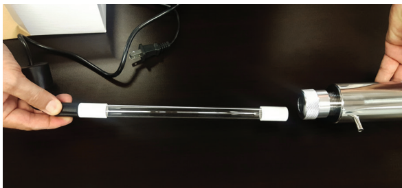
7. Carefully insert the UV lamp through the opening in the Metal Cap into the Quartz Tube.
