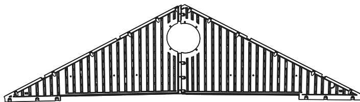
Rear Gable Assembly
