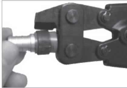
2. Cut PEX pipe close to fitting and insert small jaw inside fitting and compress handle, forcing cutter through crimp ring.
