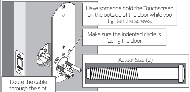
Figure B: No Mortise
