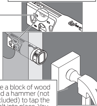
Figure B: No Mortise
