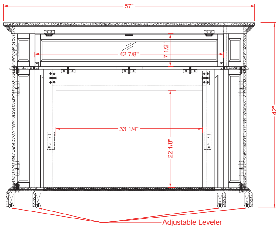
FRONT VIEW
