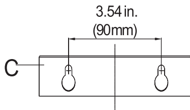
Mounting Template
