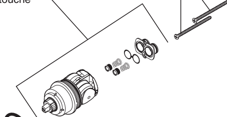
* RP46463 Cartridge Assembly Cartucho Cartouche
