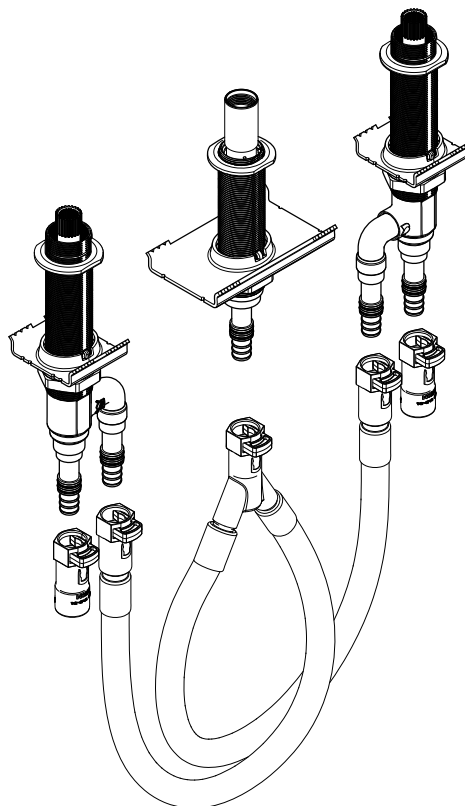
Two-Handle Roman Tub Valve with Dura-Grip™ Mounting System MODEL 4793
