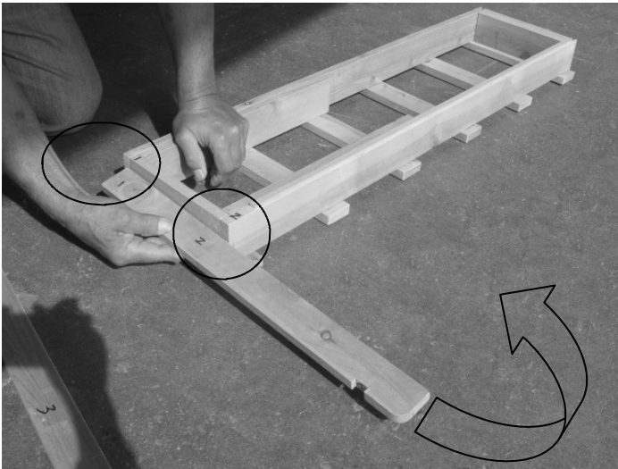
1. Assemble two bottom arbors and horizontal bench legs. Match numbers for the best result.
