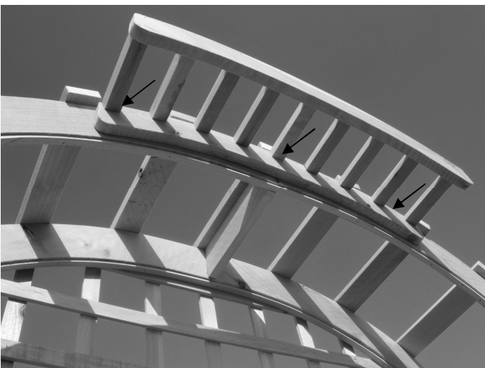
17. Fasten the crown trellis and top arbor with screws.
