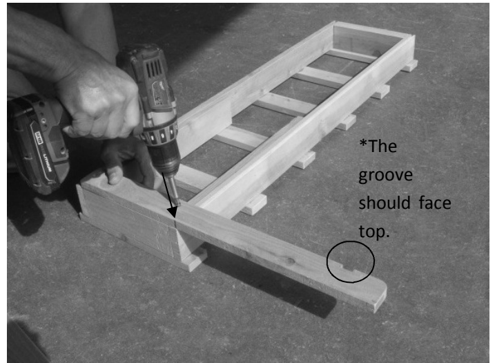
2. Flip the horizontal bench leg and fasten it to the bottom arbor with a screw.
