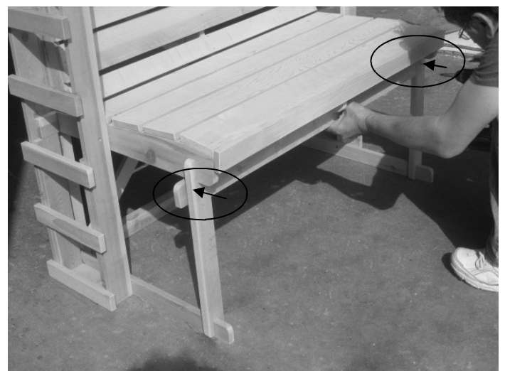
12. Fasten the horizontal bench support under the bench. Match numbers for the best result and fasten them with screws.
