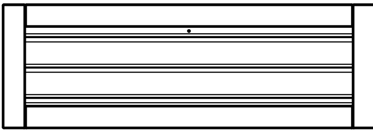
(1) WP6 - PANEL POSTERIOR DE PARED - W2A01765 1 1/8"x39 1/8"x13" (27x994x330)
