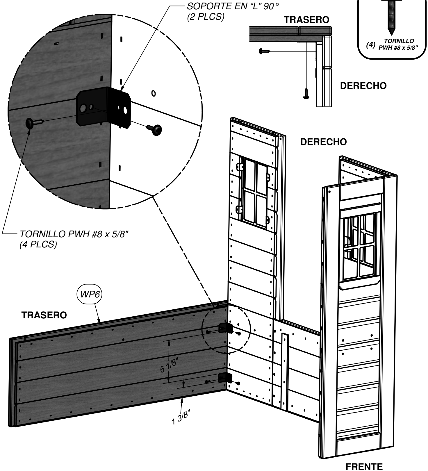
(1) WP6 - PANEL POSTERIOR DE PARED - W2A01765 1 1/8"x39 1/8"x13" (27x994x330)
