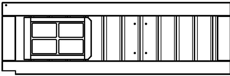
(1) WP1 - PANEL DELANTERO IZQUIERDO DE PARED - W2A01759 1 1/8"x12 5/8"x39 7/8" (27x320x1014)
