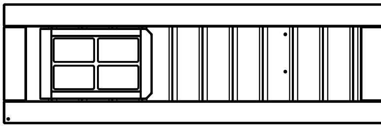
WP4 - PANEL DE PARED LADO DERECHO DERECHO - W2A01763 (1) 1 1/8"x12 5/8"x39 7/8" (27x320x1014)
