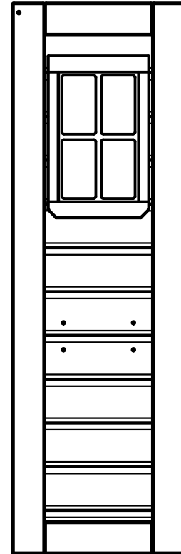
WP2 - PANEL DE PARED FRONTAL DERECHA - (1) W2A01760 1 1/8"x12 5/8"x39 7/8" (27x320x1014)
