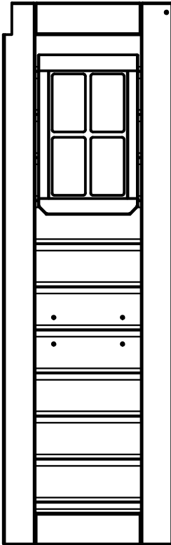
WP1 - DELANTERO IZQUIERDO PANEL - (1) W2A01759 1 1/8"x12 5/8"x39 7/8" (27x320x1014)
