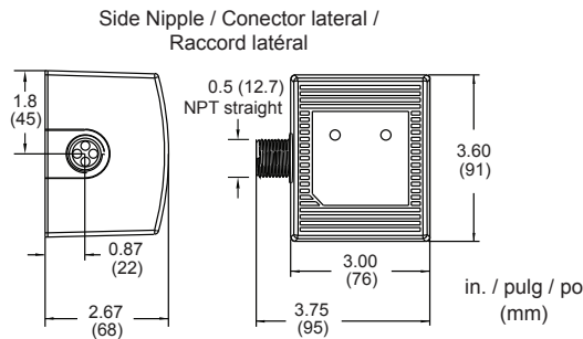
Figure / Figura / Figure 4 : Dimensions / Dimensiones / Dimensions
