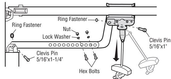
One-Piece Door with Track
