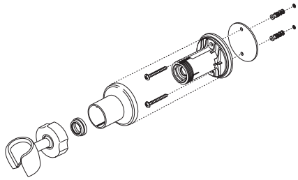
RP61294▲ Mounting Bracket Consola de montaje Support
