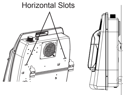
Fig. 19b - Mounting Heater Onto Mounting Bracket
