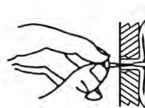
Fig. 18 - Popping Open Anchor Wing For Thin Walls
