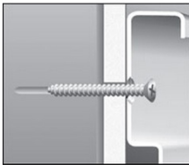
Studs Secure to the wall with #12 x 2" pan head screws at stud locations.
