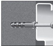
Concrete Drill 1/4" holes. Insert #12 wall anchors and secure to the wall with #12 x 2" pan head screws.
