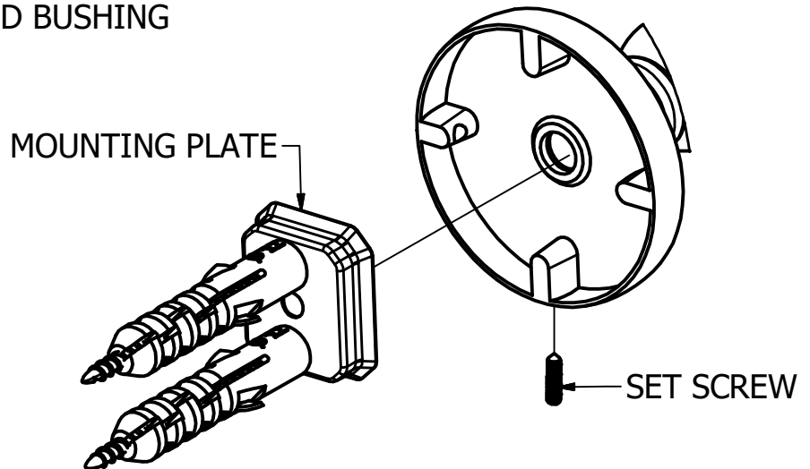
DETAIL D
