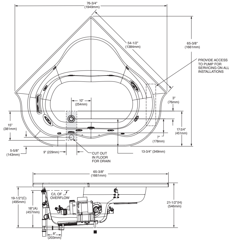
DIMENSIONS OF FIXTURES ARE NOMINAL AND MAY VARY WITHIN THE RANGE OF TOLERANCES ESTABLISHED BY ANSI STANDARDS Z124.1 AND A112.19.7
