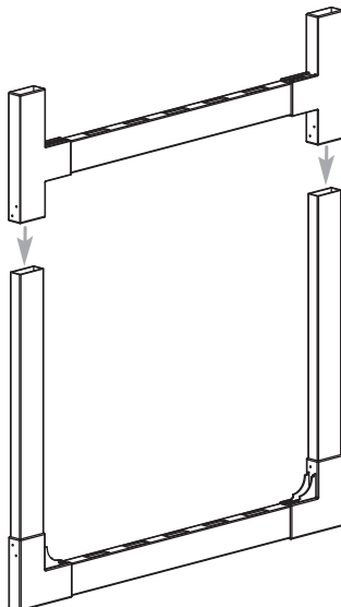
E - Slide brackets with toprail attached down over the vertical gate stiles
