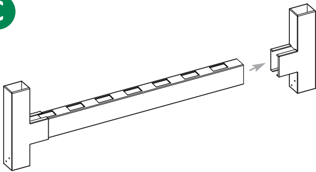
C - Insert rail until it bottoms out inside bracket (glue first)
