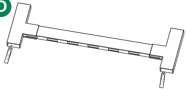
D - Run a bead of vinyl-weld continuously around the inside of the brackets
