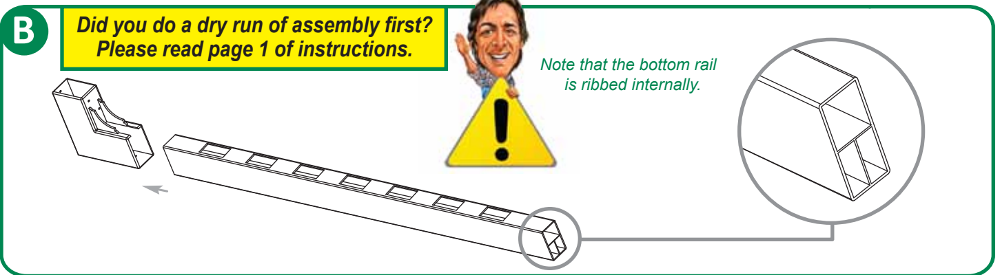
B - Insert the bottom rail until it bottoms out inside gate bracket
