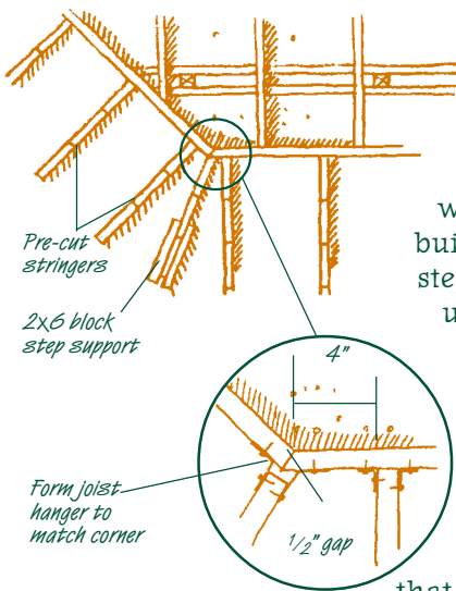
Wraparound Stair Detail
