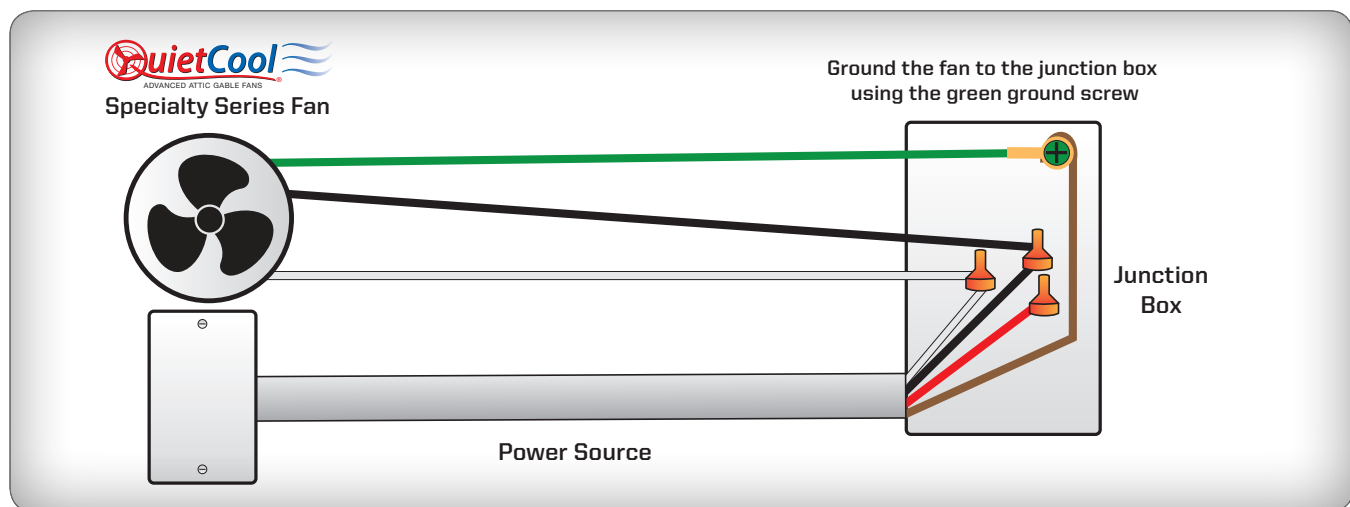
Figure 3.1A: Smart Attic Fan at the Junction Box
