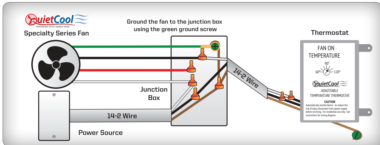
Figure 3.2D: Thermostat Wiring in a Remote Location - Low Speed
